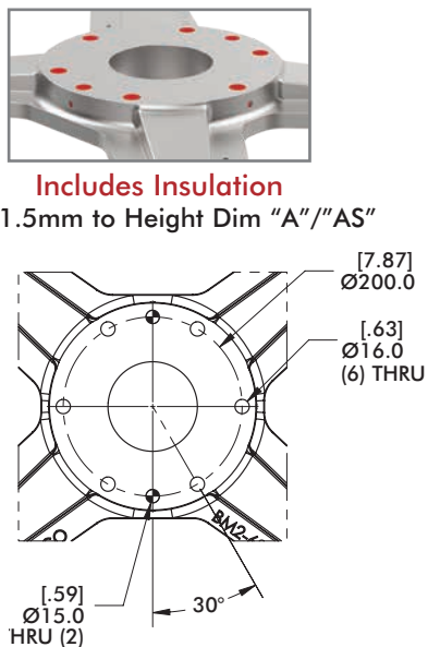
R16 (Ø200mm Bolt Circle)
